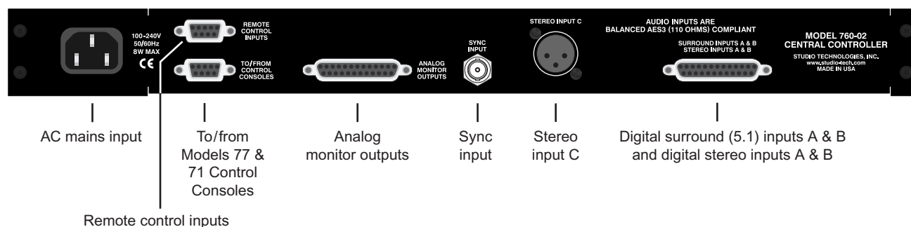
Figure 2. Model 760-02 Central Controller Back Panel
