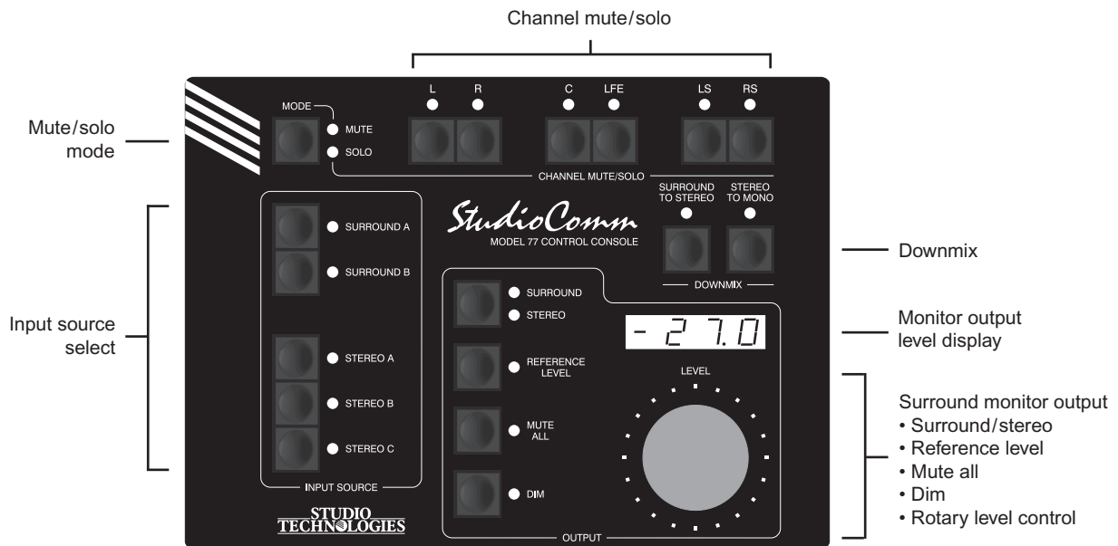
Figure 3. Model 77 Control Console Front Panel
